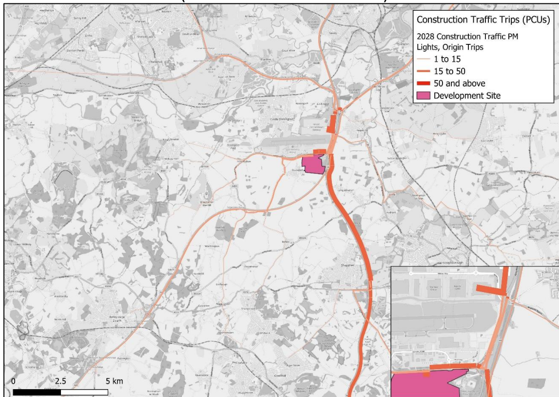
Figure 2.4: 2028 Car, Van and Light Vehicle Trip Distribution (PM)
